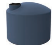
BT3000-S 3,000L/660Gal (Squat) Height 1,500mm Diameter 1,800mm Outlet 25mm Overflow 90mm
